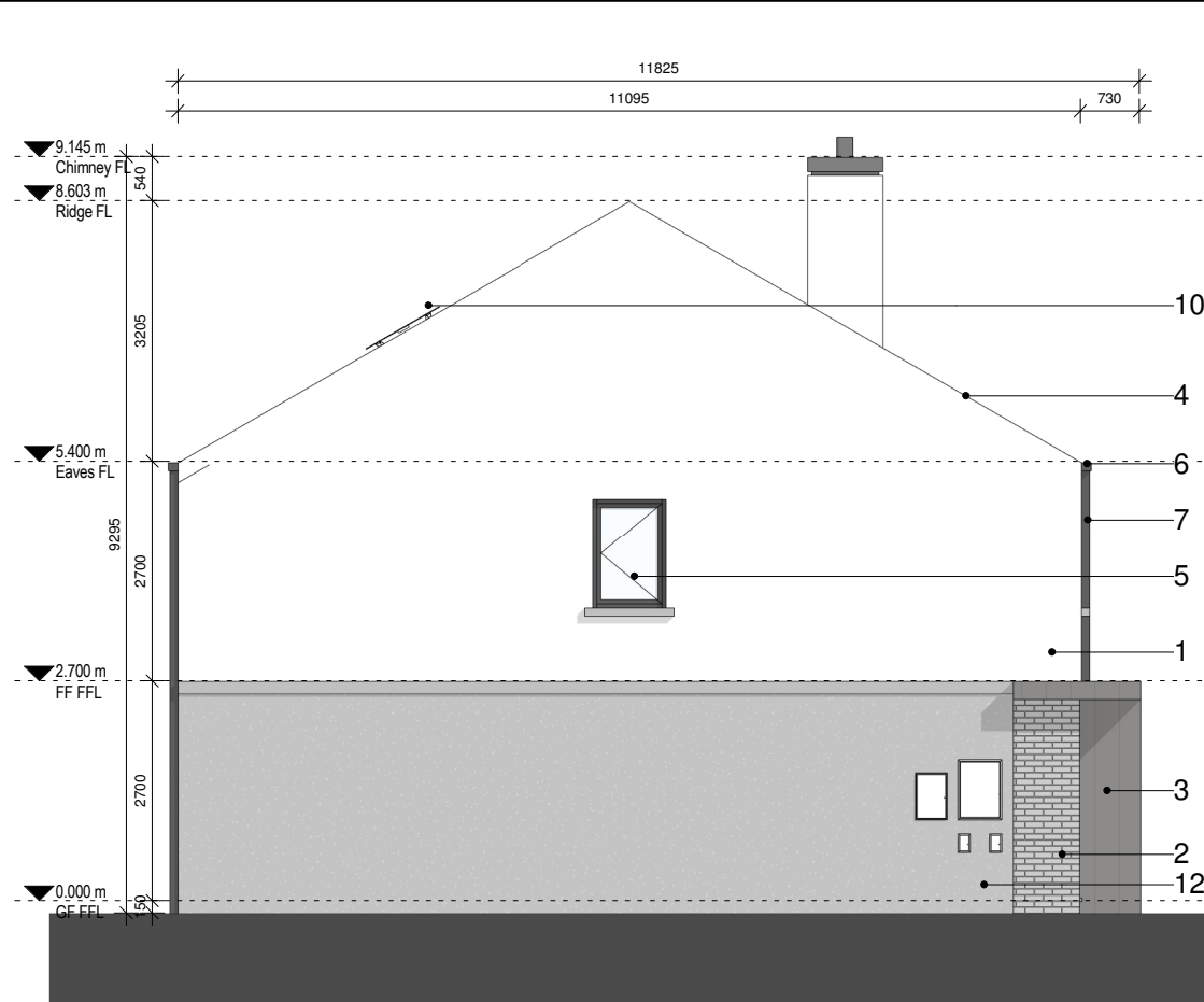
2 02 Side Elevation 1: 100 @ A3
