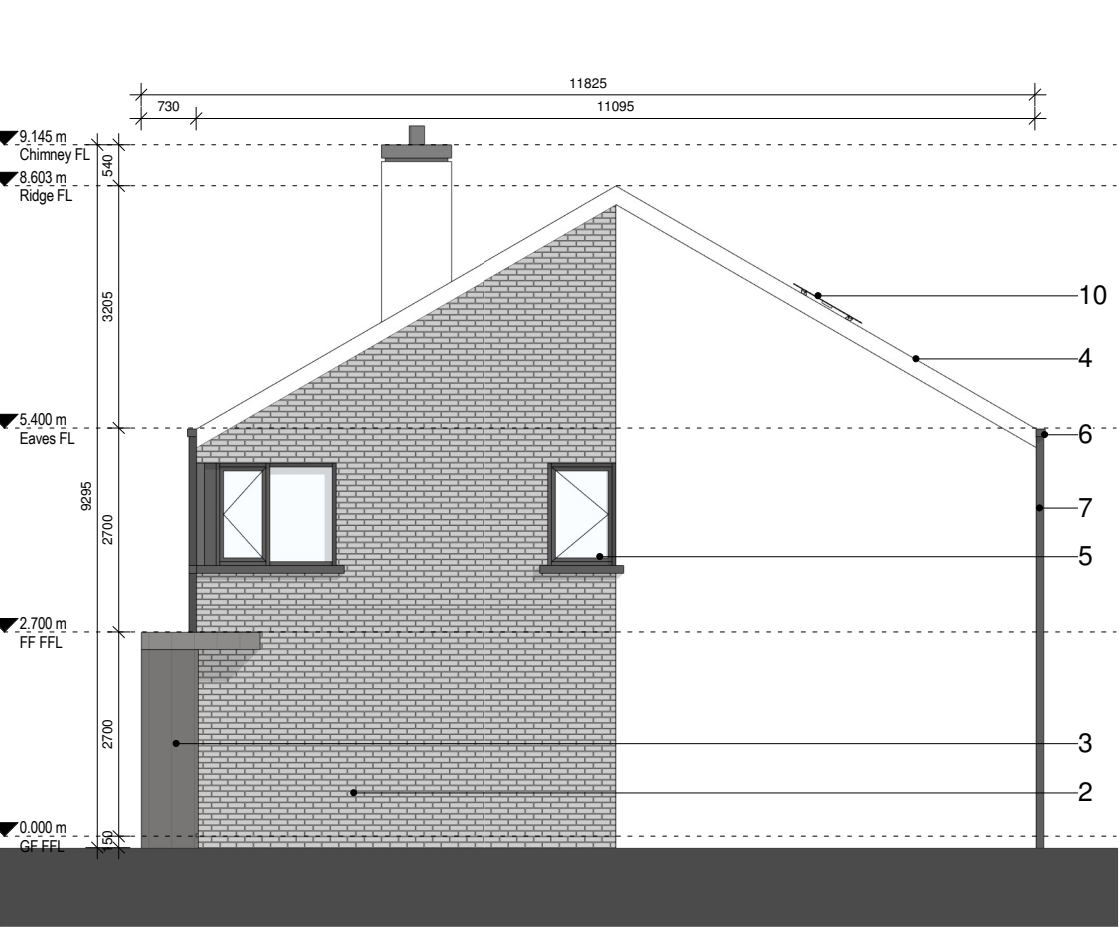
4 04 Side elevation 1: 100 @ A3
